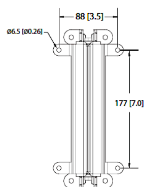
Wall-Mount Section
