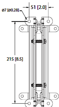
Loudspeaker-Mount Section
