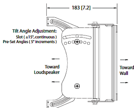
Assembled Bracket
